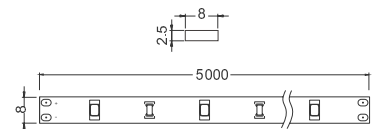
IP20 MODELS
